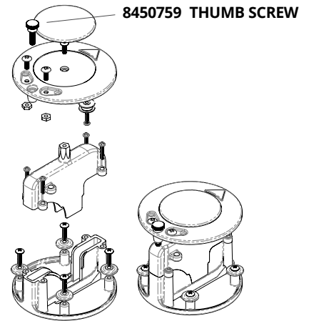
8450759 THUMB SCREW
